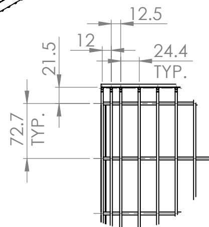
DETAIL D SCALE 1 : 5
