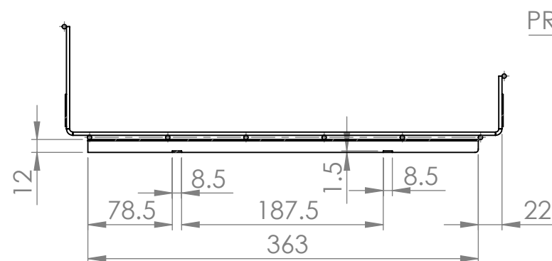
SECTION C-C SCALE 1 : 5
