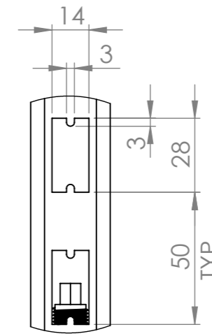
DETAIL A SCALE 1 : 2
